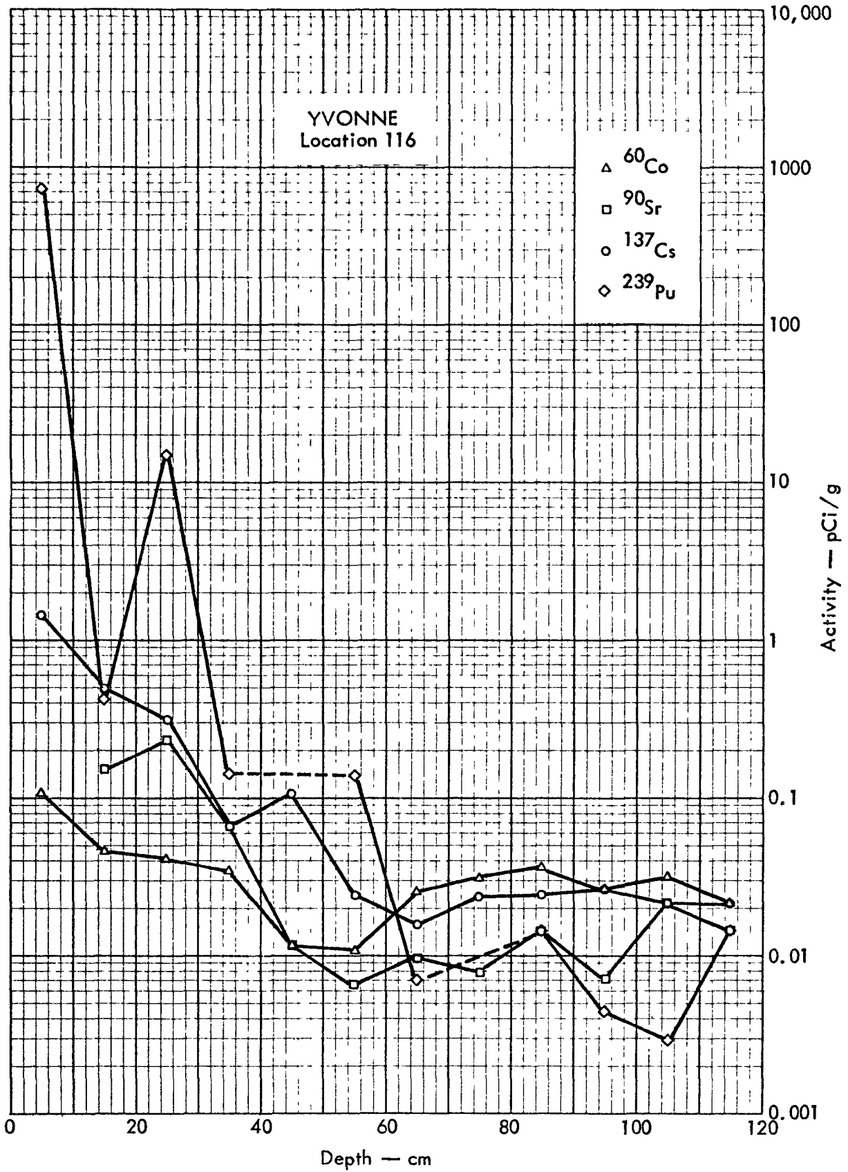
FIGURE 95. ACTIVITIES OF SELECTED RADIONUCLIDES AS A FUNCTION OF SOIL DEPTH
